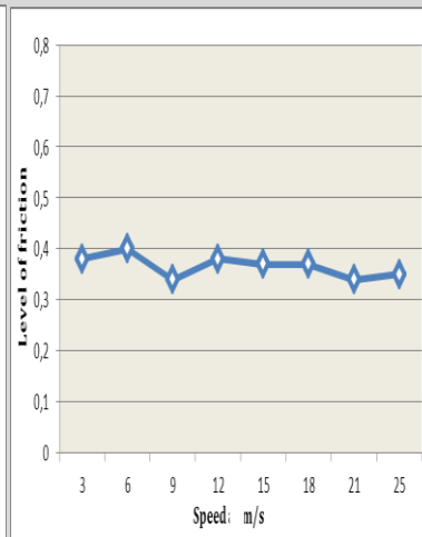
Friction dependent the speed at 6 bars
