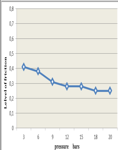
Friction dependent Pressure
