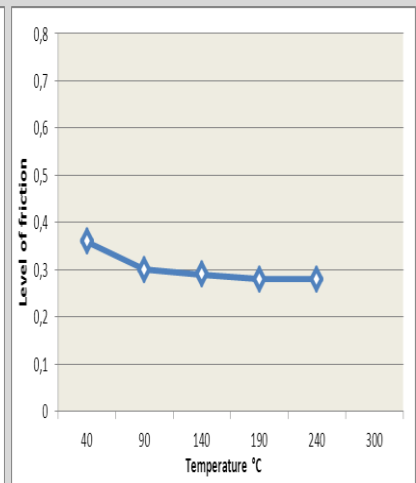
Friction dependent Temperature
